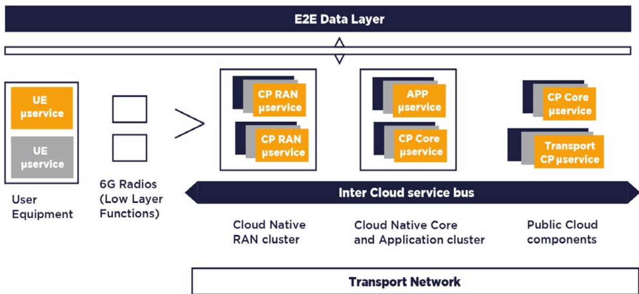
Figure 3-2. 6G Intelligent Open Network concept.
